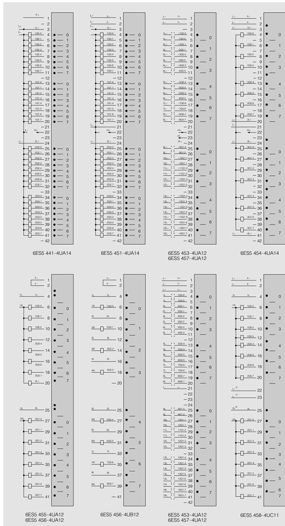
Fig. 4/24 Connection diagrams of digital output modules
