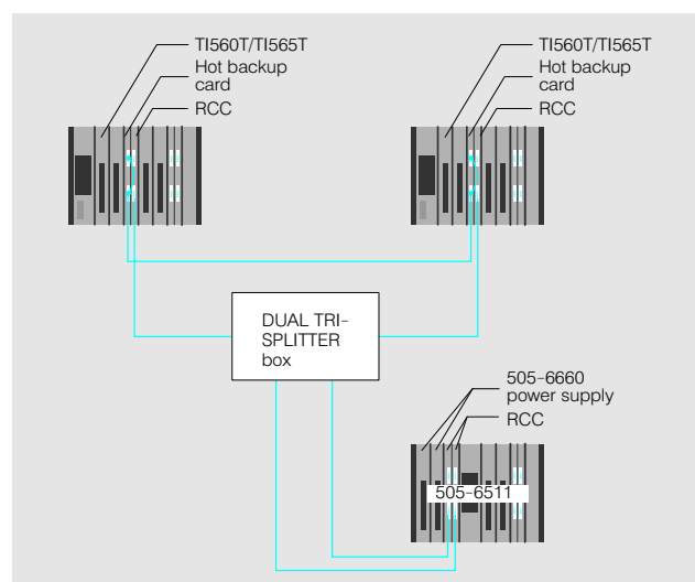
Fig. 5/3 Hot backup with two-channel I/O
