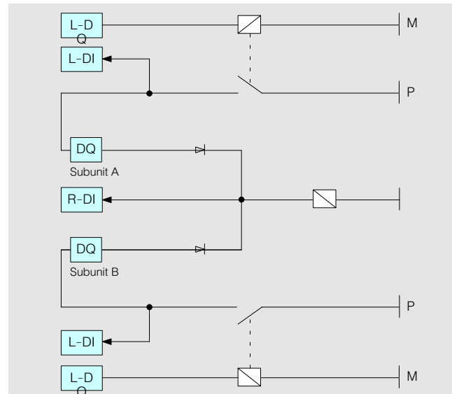
Fig. 11/4 Redundant, intermittent digital output with fault location
