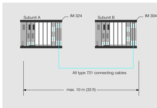
Fig. 3/40 Interfacing of central controllers
