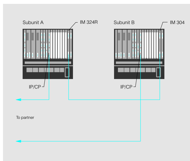
Fig. 4/20 CP/IP in two-channel redundant configuration
