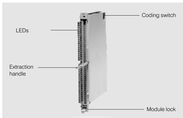
Fig. 4/5 Design of the I/O modules
