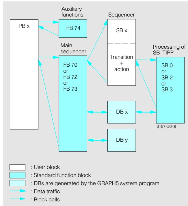
Fig. 7/31 Calling structure
