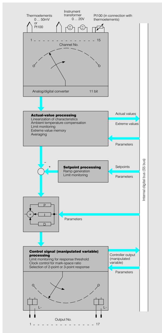
Fig. 4/33 Function diagram of temperature control module
