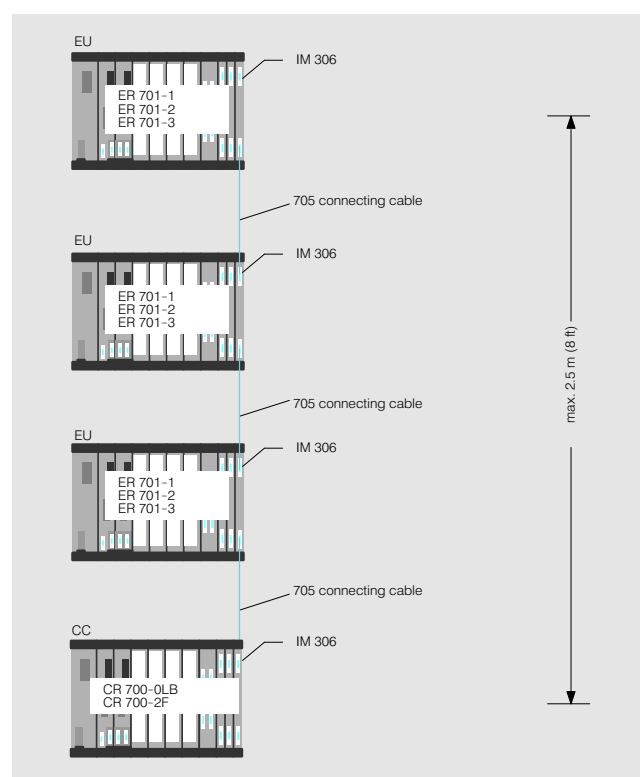
Fig. 3/41 Central configuration of expansion units with IM 306 (1 subunit)
