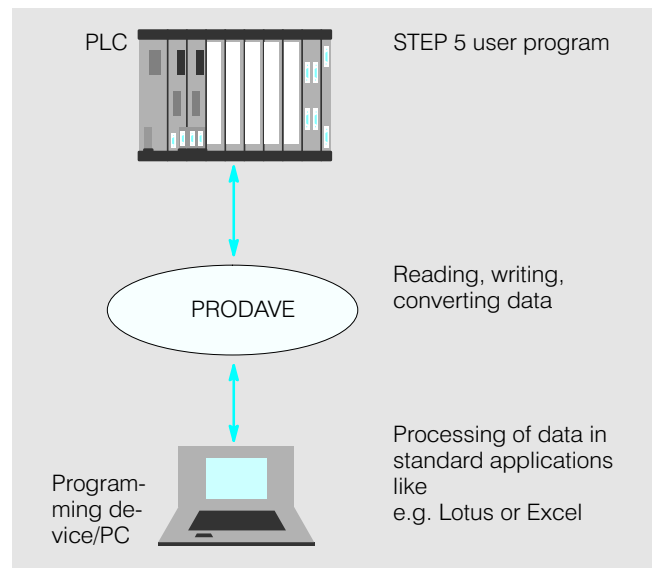
Fig. 7/11 Programming with PRODAVE
