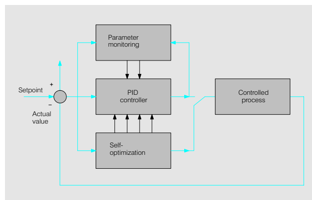
Fig. 4/34 Function diagram of controller self-optimization
