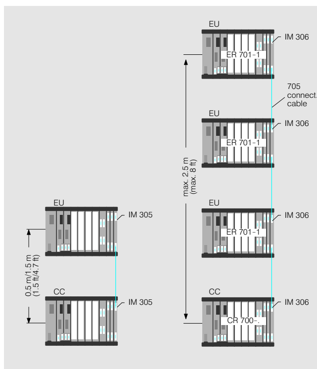
Fig. 3/33 Connection of expansion units to the central controller in centralized configuration using IM 305 (left) and IM 306 (right) interface modules
