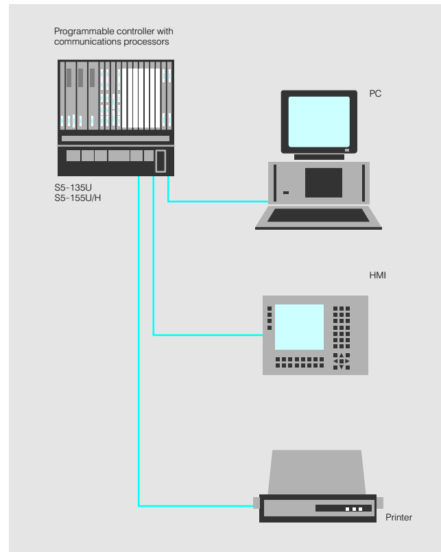
Fig. 4/11 Interfacing the programmable controller with PC, HMI devices and printer
