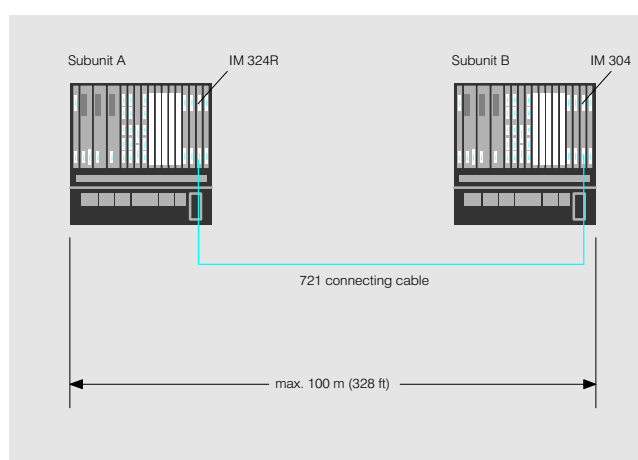
Fig. 4/56 Interfacing of the two central controllers
