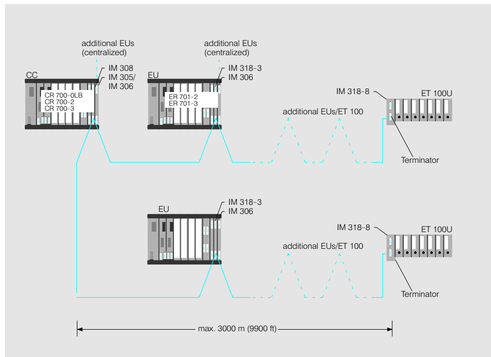
Fig. 3/37 Connection of expansion units and ET 100U electronic terminators to the central controller in distributed configuration using IM 308 and IM 318 interface modules
