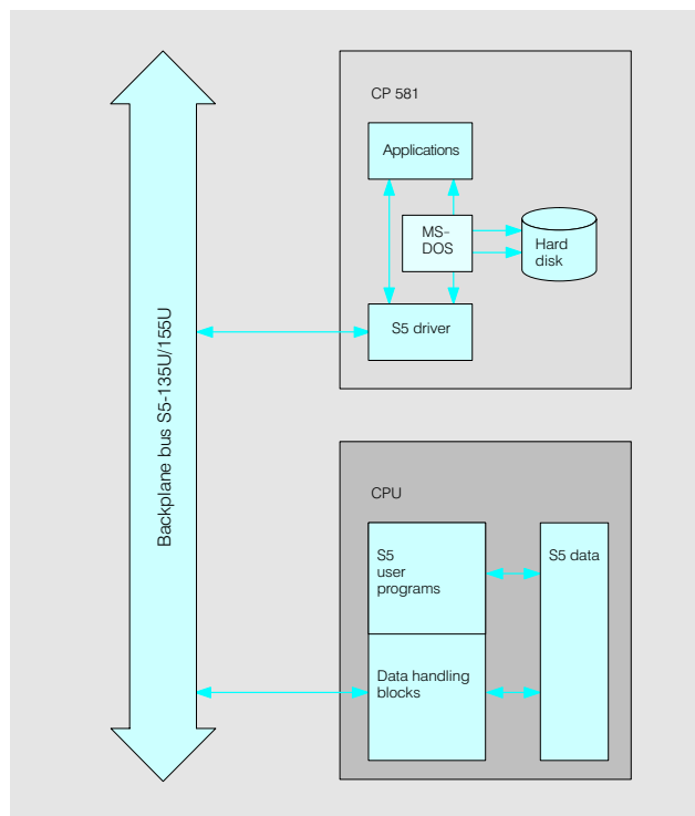
Fig. 4/44 Data exchange between CP 581 and CPU
