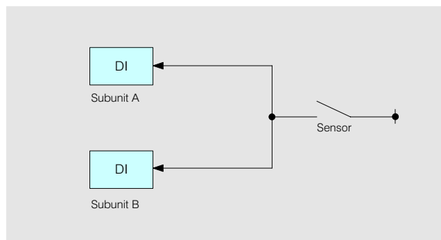
Fig. 11/6 Double-redundancy digital input without fault location
