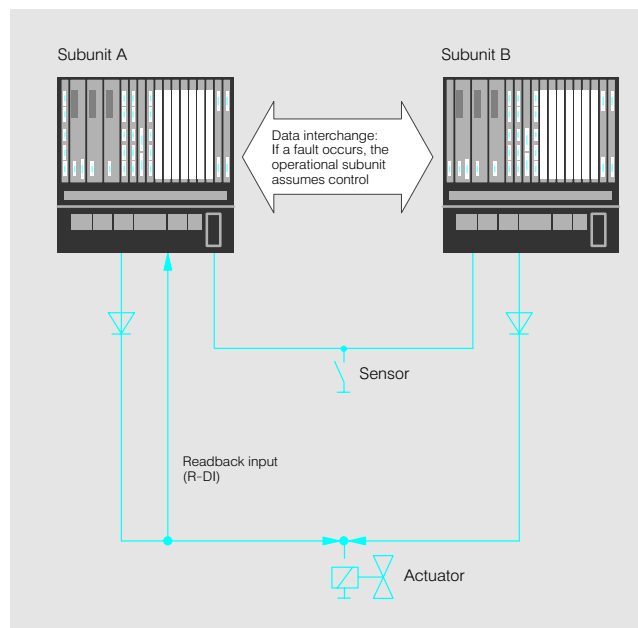
Fig. 4/21 Example of an S5-155H with redundant input and output
