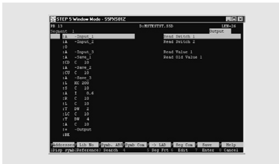
Fig. 7/2 STEP 5, STL representation
