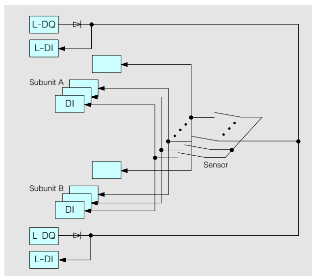
Fig. 11/7 Double-redundancy digital input with fault location
