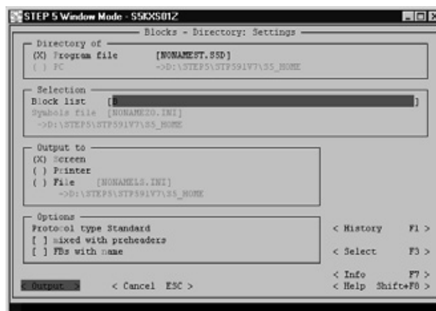
Fig. 7/4 Dialog field-structure
