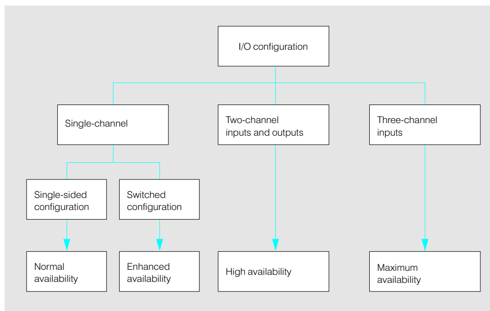
Fig. 4/13 Degrees of availability of the I/O area
